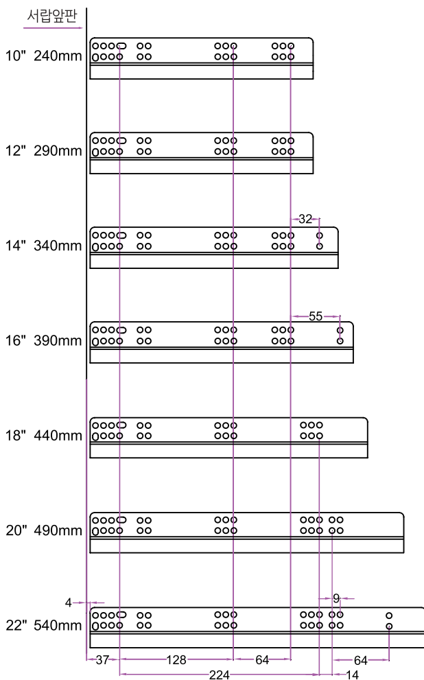
측판레일도면 | Drawing
